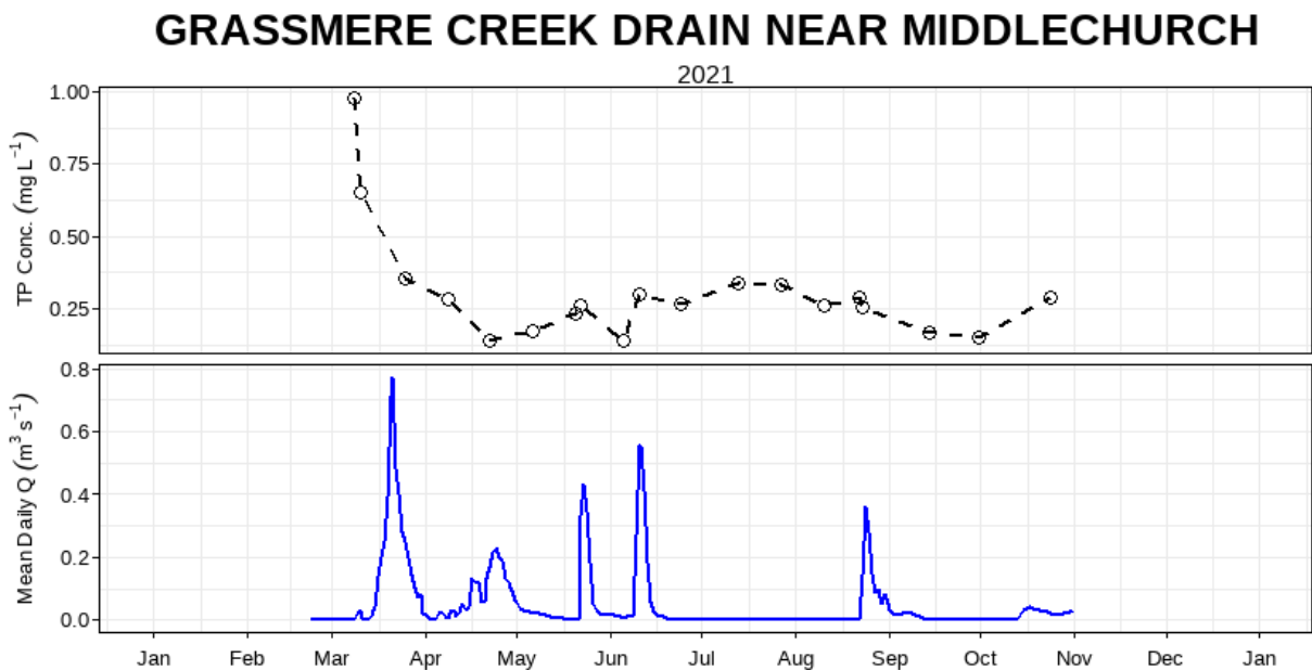
Figure 6: Mean daily discharge (m 3 s -1 ) and total phosphorus concentration (mg L -1 ) over the 2021 sampling season at Grassmere Creek Drain near Middlechurch (05OJ017).
