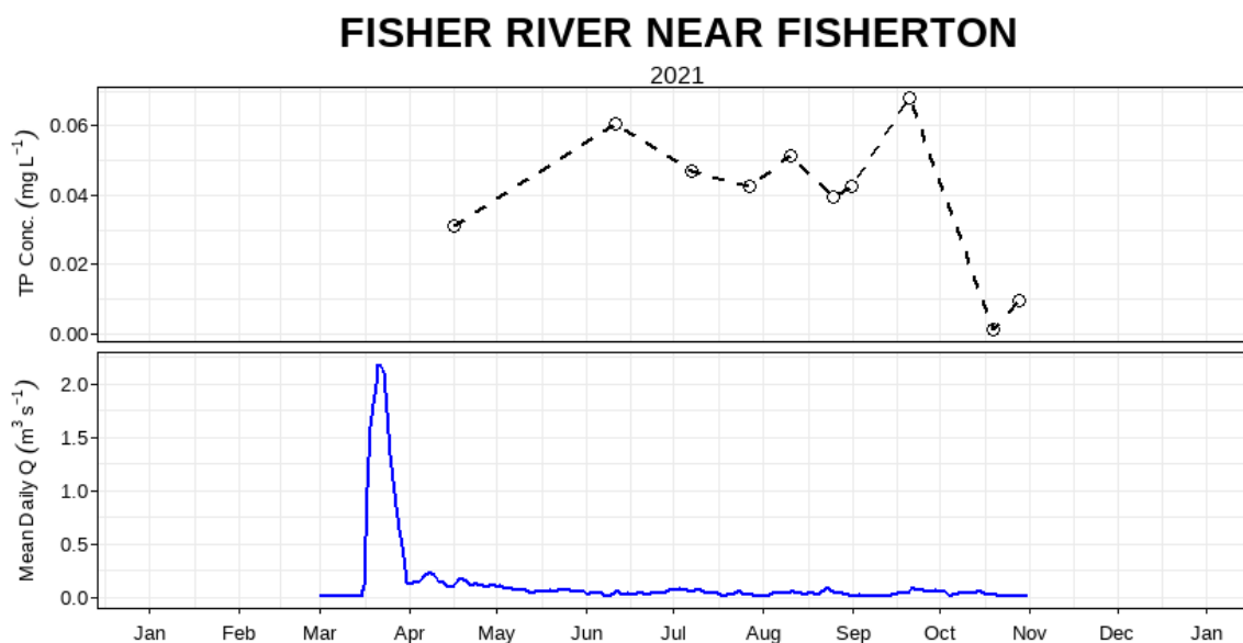
Figure 4: Mean daily discharge (m 3 s -1 ) and total phosphorus concentration (mg L -1 ) over the 2021 sampling season at Fisher River near Fisherton (05SD005).
