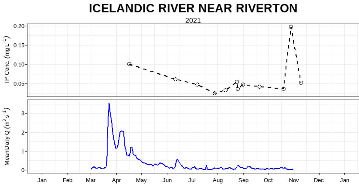
Figure 8: Mean daily discharge (m 3 s -1 ) and total phosphorus concentration (mg L -1 ) over the 2021 sampling season at Icelandic River near Riverton (05SC002).
