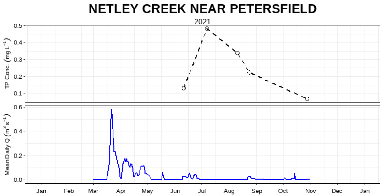
Figure 10: Mean daily discharge (m 3 s -1 ) and total phosphorus concentration (mg L -1 ) over the 2021 sampling season at Netley Creek near Petersfield (05OJ008).
