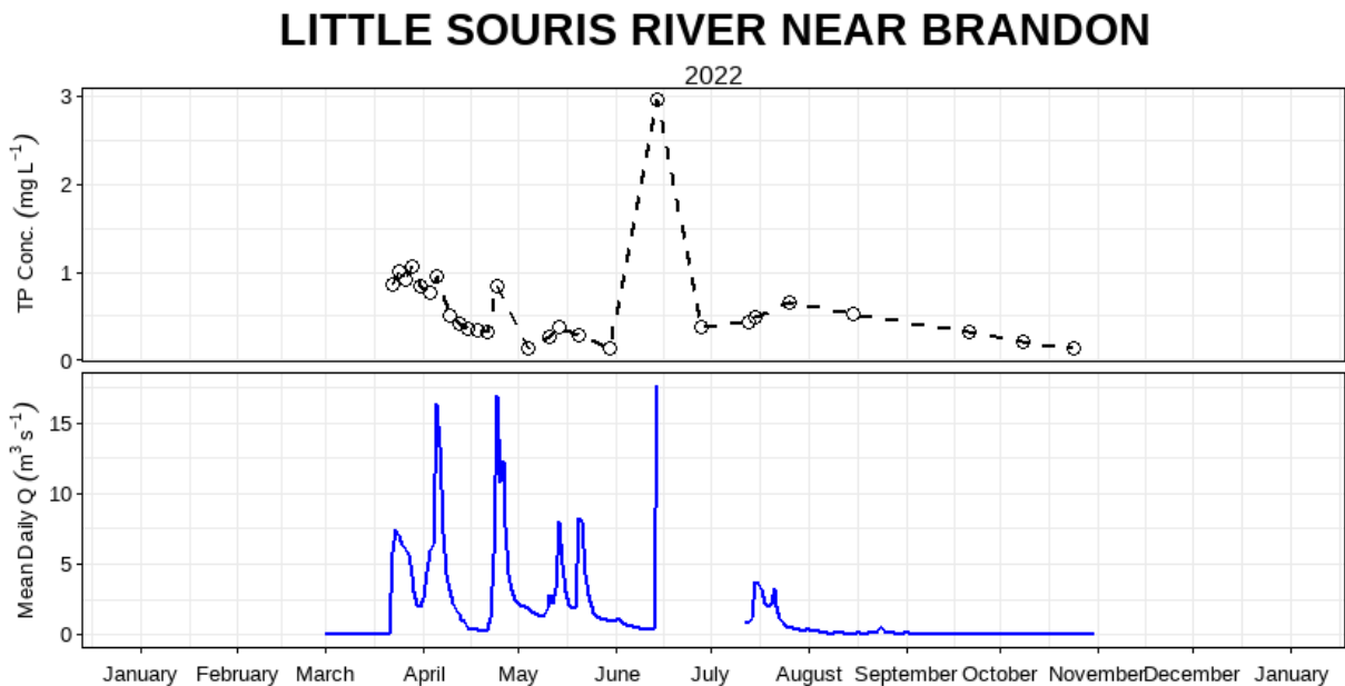
Figure 6: Mean daily discharge (m 3 s -1 ) and total phosphorus concentration (mg L -1 ) over the 2022 sampling season at Little Souris River near Brandon (05MH006).
