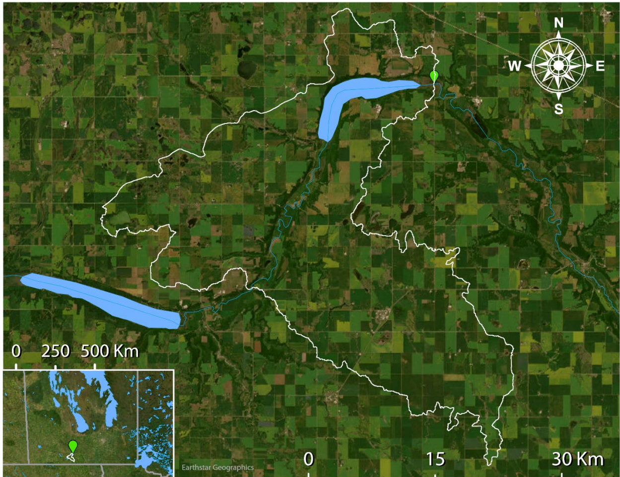
Figure 17: WSC station 05OB019 (green), and incremental drainage area polygon (white - source: WSC). See Supplemental Figure 2 Supplemental Figure 3 for upstream drainage areas used to calculate incremental area. LWCBMN samples directly at the WSC station.
